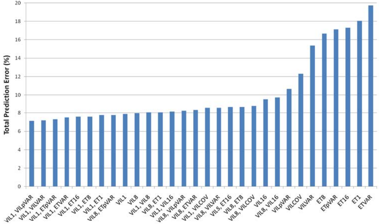
Figure 4. Total predictor error of the full set of 1- and 2-predictor classifiers.
