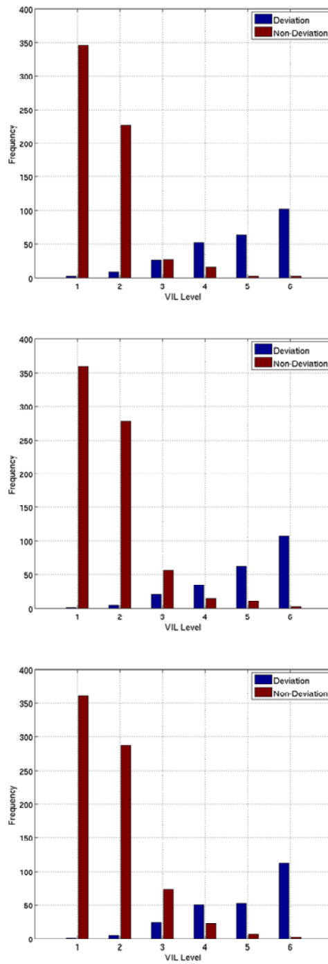
Figure 8. Deviation/non-deviation histograms. Top: 1 km spatial filter. Middle: 8 km spatial filter. Bottom: 16 km spatial filter.
