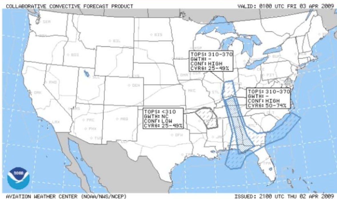
Figure 5-17 Example of the Collaborative Convective Forecast Product. ( www.aviationweather.gov )
