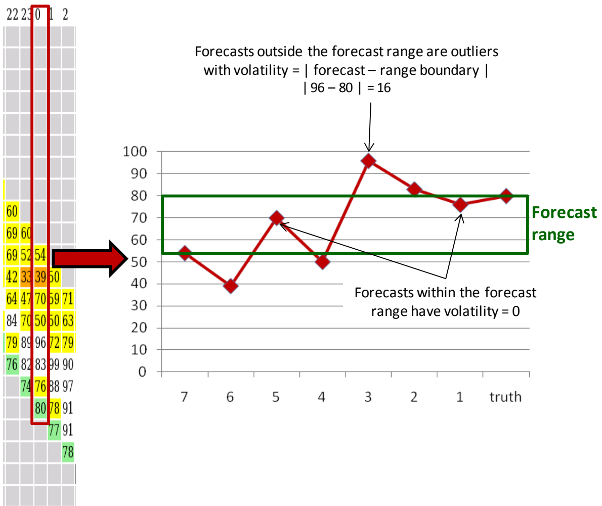
Figure 16. Illustration of the forecast volatility metric.
