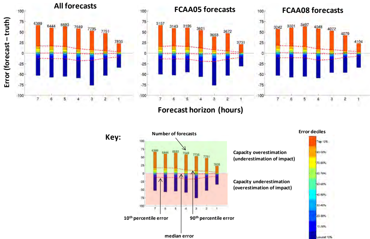
Figure 12. Comparison of Matrix capacity forecast error for different FCA boundaries.
