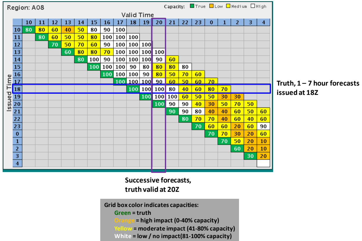
Figure 2. Illustration of the capacity Matrix output.
