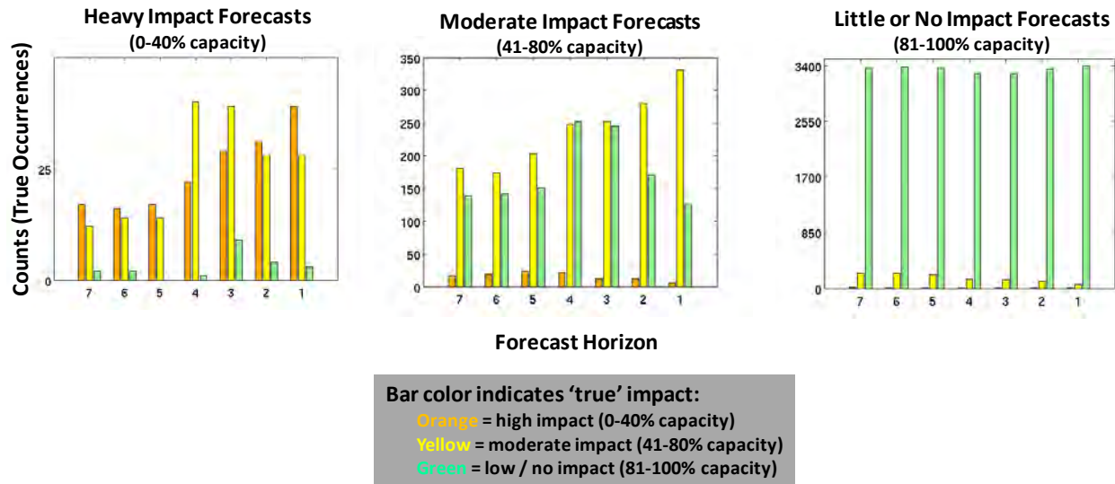
Figure 18. Histogram of Matrix capacity forecast accuracy when forecasting capacity impact ranges.
