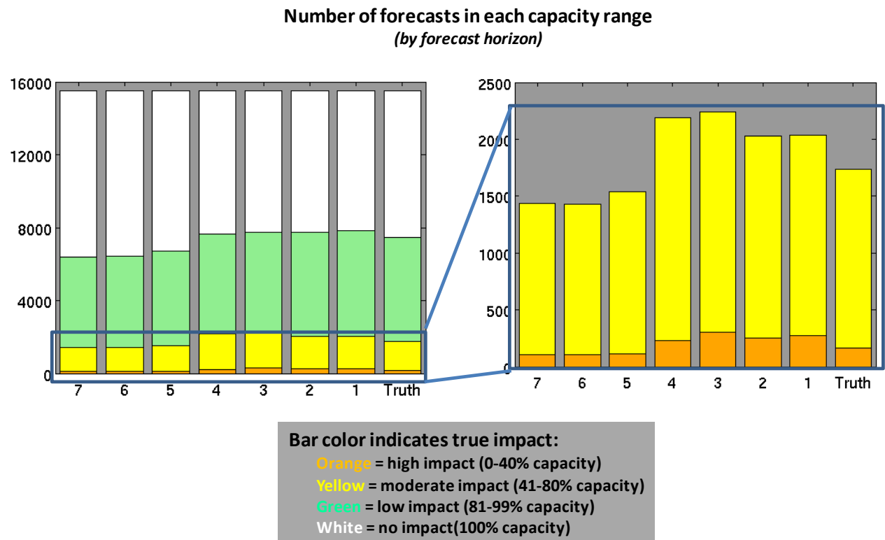
Figure 7. Distribution of Matrix capacity forecasts by impact range. The figure at right is an expanded view of the distribution of just the moderate and high impact forecasts.
