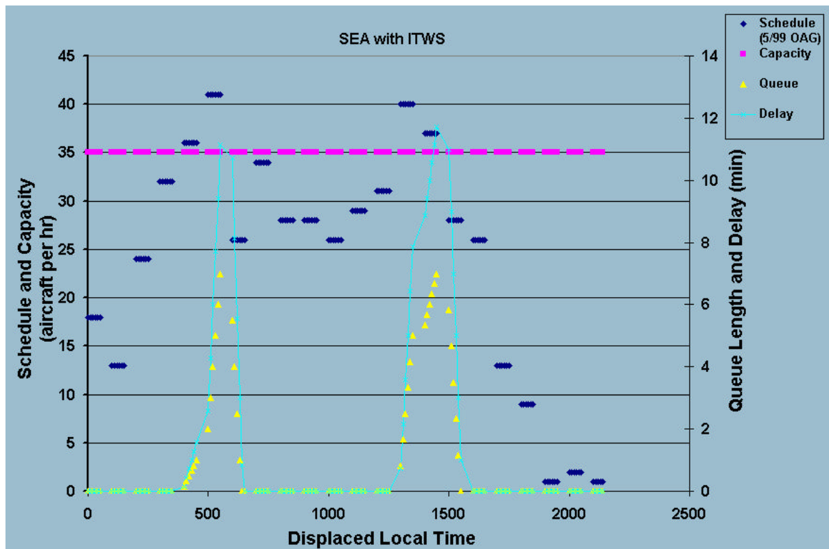
Figure E-6. SEA delays assuming that ITWS permits landing 35 aircraft per hour.
