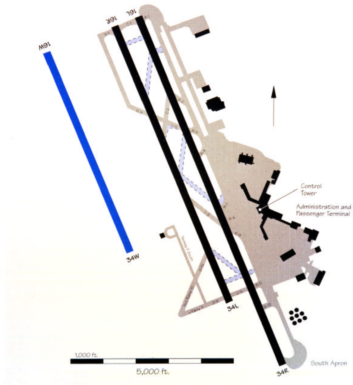
Figure 19. SEA Airport Layout. Blue indicates runway under construction. (from US DOT FAA “1998 Aviation Capacity Enhancement (ACE) CD-ROM and Airport Database”)
