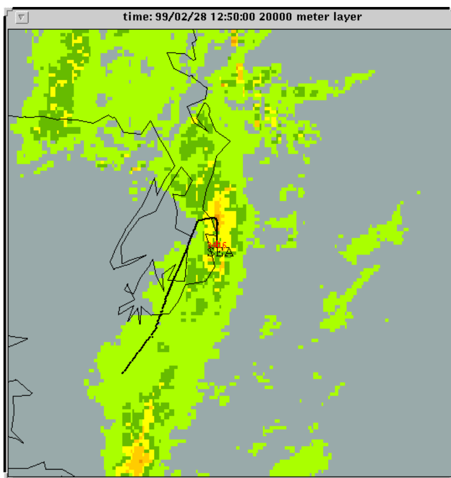
Figure C-2. Track of Flight NWA946. The SEATAC airport is labeled with the letters “SEA” and the red portion of the track indicates the position of the aircraft at the time of the lightning strike.
