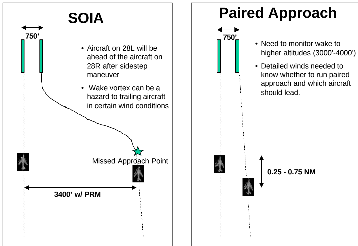
Figure 15. SFO parallel approach (Figure from T.J. Dasey, 23 June 1999 briefing to AND 400).
