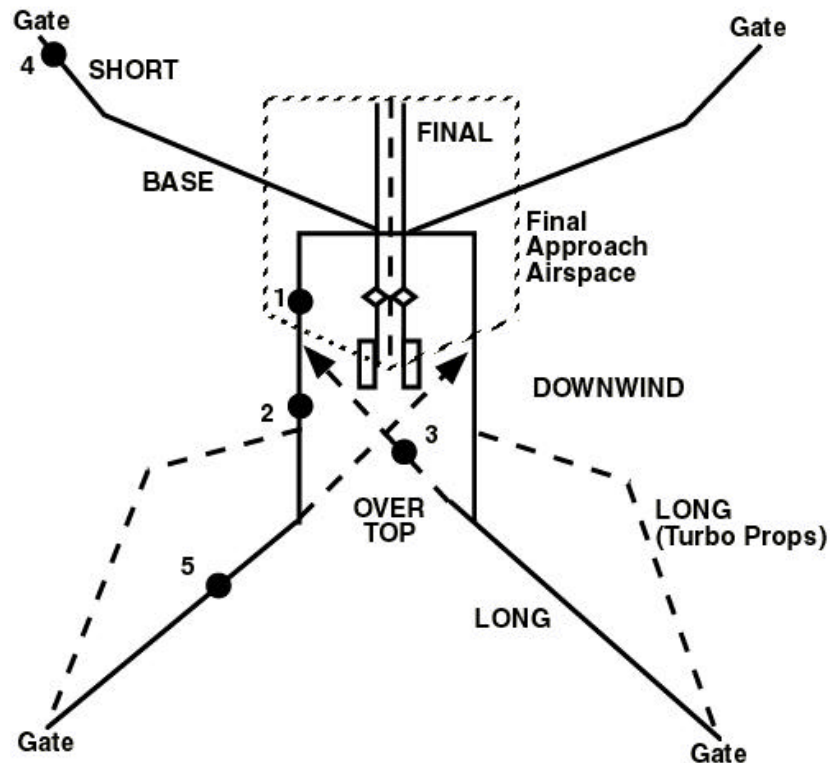
Figure 3. Aircraft being sequenced to left runway are denoted by a numbered ●.
