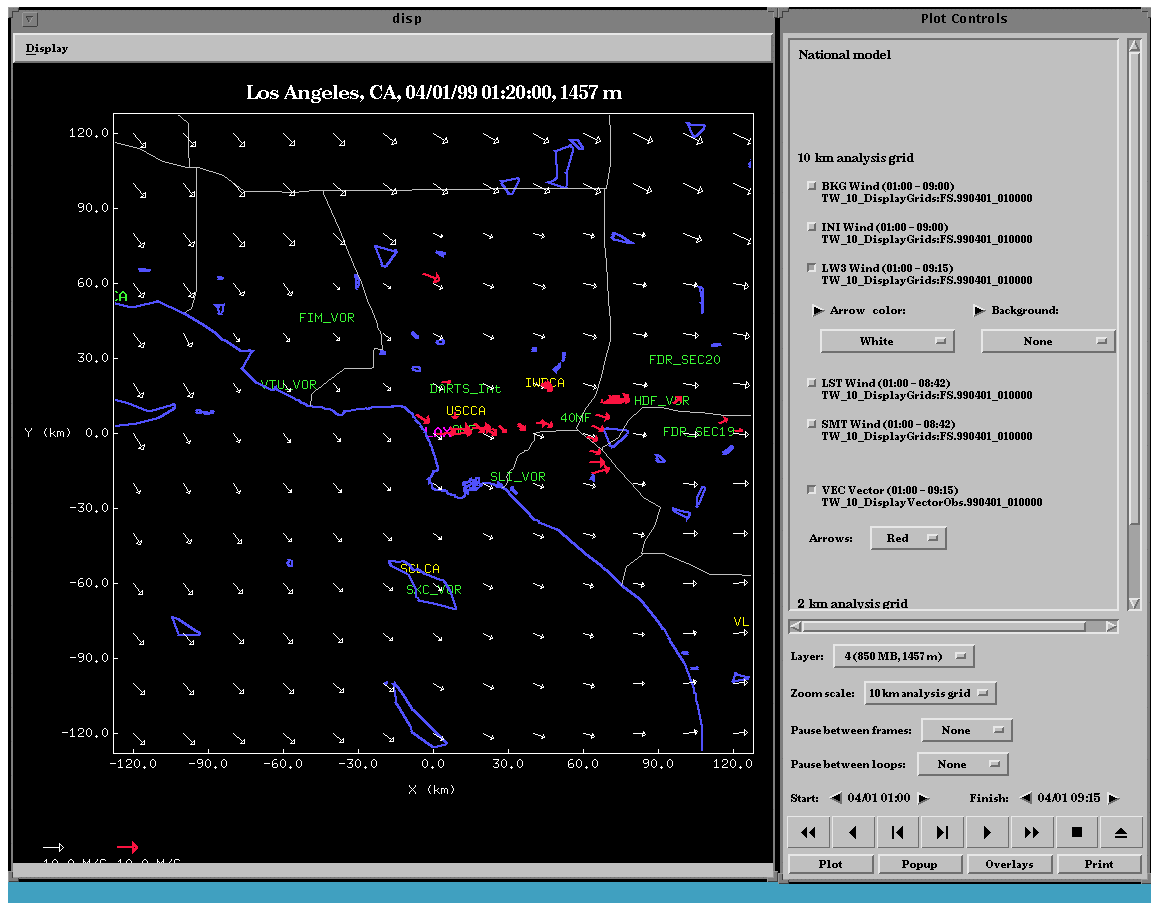
Figure 17. LAX Terminal Winds at 4500 ft. The white arrows are the horizontal gridded wind estimates on a 10 km grid. The yellow text indicates the locations of wind profilers, the red arrows indicate MDCRS reports from a 30-minute period. The length of arrows at the bottom left indicate a 10 m/s wind velocity. The green text indicates ATC fixes for the SoCal TRACON.
