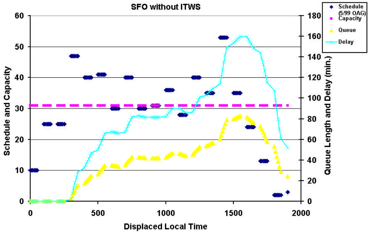
Figure E-3. SFO delays assuming landing 31 aircraft per hour.
