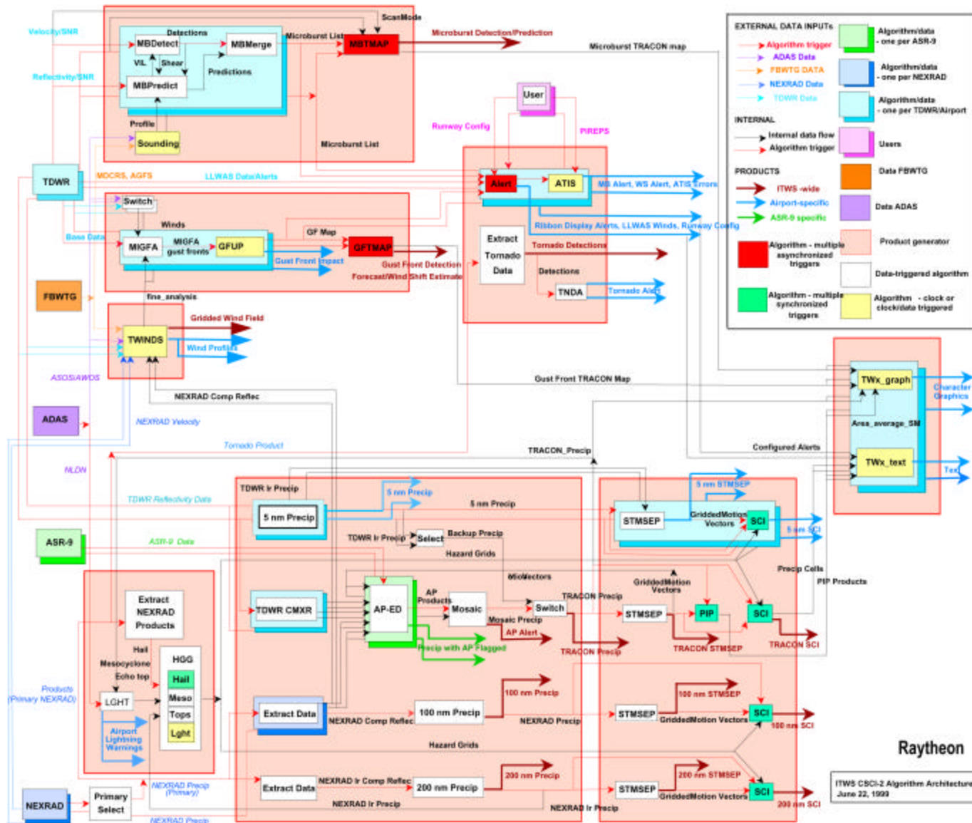
Figure 5. IOC ITWS Computer Software Configuration Item (CSCI) architecture (graphic from Raytheon, Sudbury, MA).
