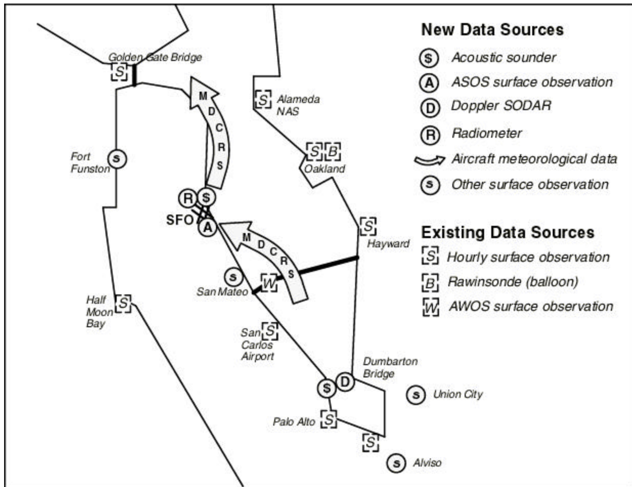
Figure 14. Locations of data sources in San Francisco Bay area.
