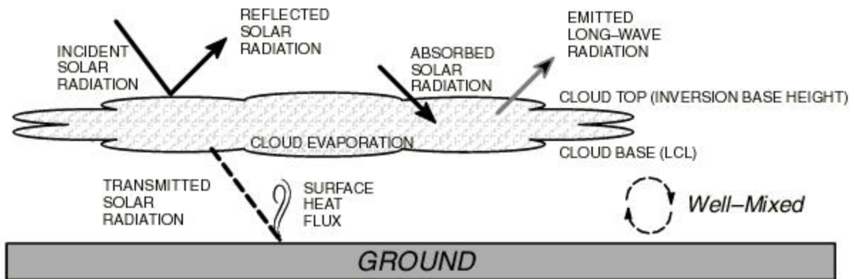
Figure 9. Key meteorological parameters for coastal stratus prediction.
