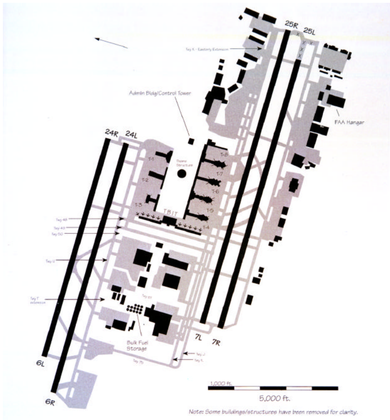
Figure 16. LAX Airport Layout (from US DOT FAA "1994 Aviation Capacity Enhancement (ACE) Plan," DOT/FAA/ASC-94-1, Appendix E-25).
