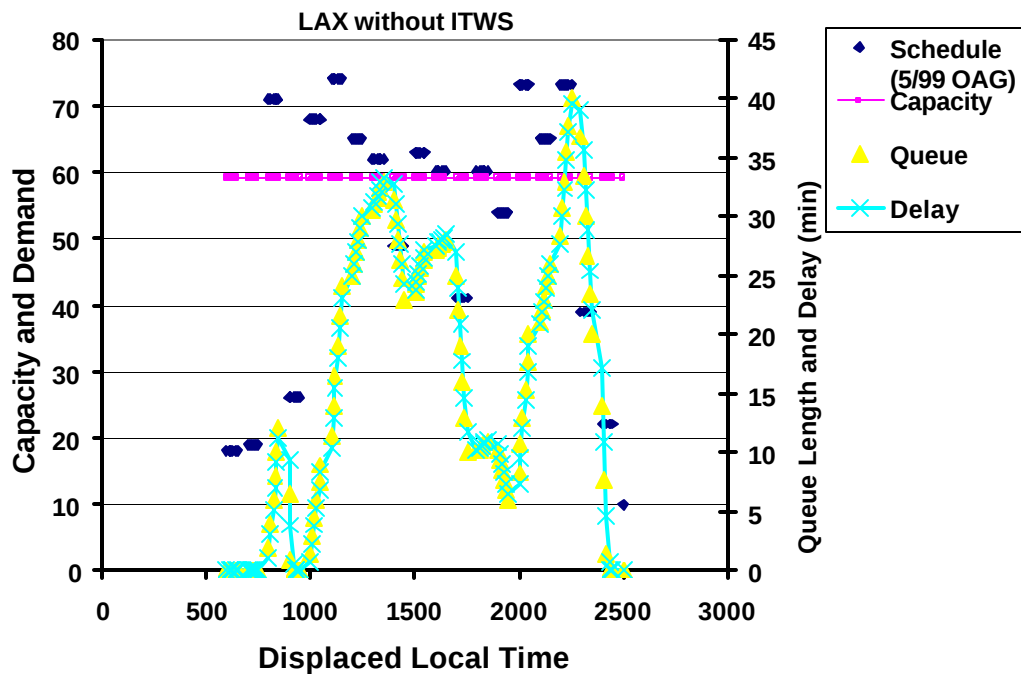
Figure E-1. LAX delays landing 59 aircraft per hour.
