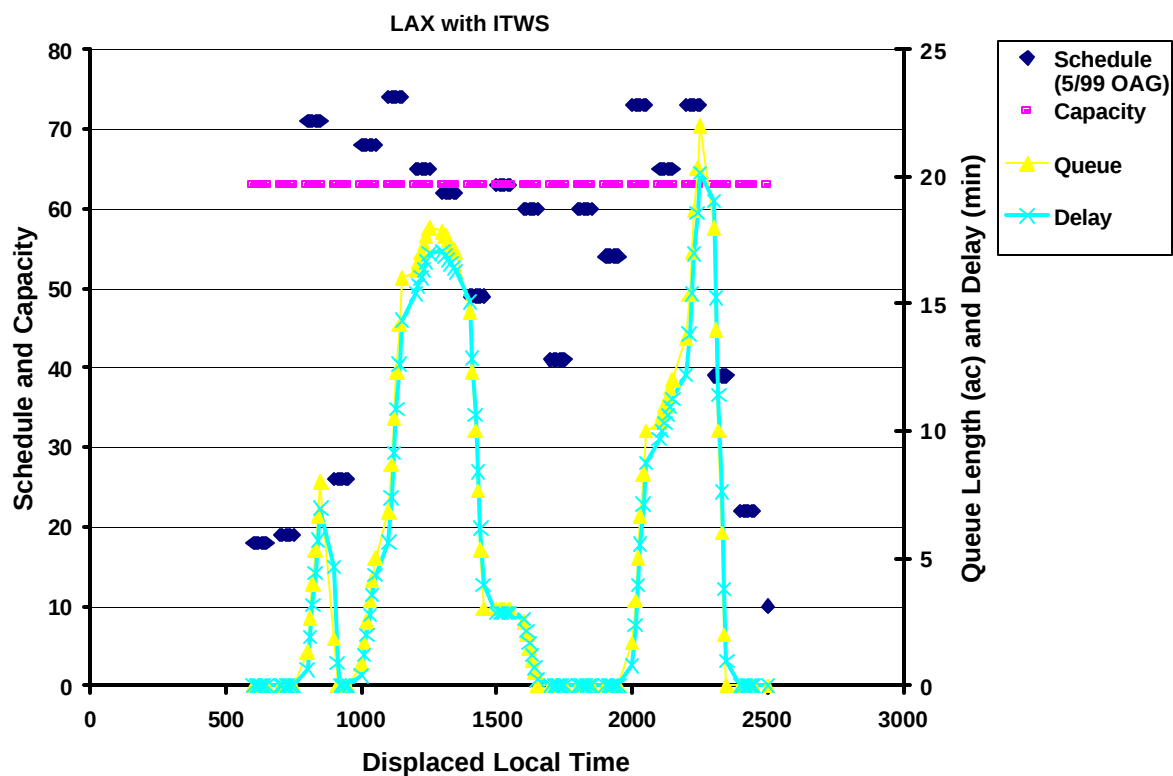
Figure E-2. LAX delays assuming ITWS terminal winds permits landing 63 aircraft per hour.
