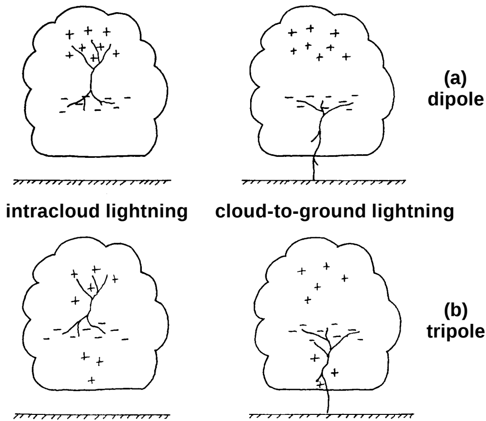
Figure G5. Depiction of intracloud and cloud-to-ground lightning in prototype electrostatic structures: (a) dipole and (b) tripole (from Williams, et al., 1998).
