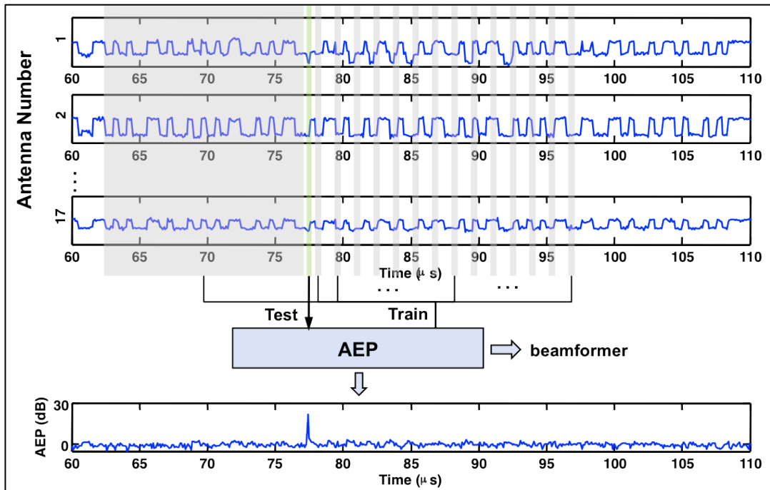
Figure 3-14. Simulated SSPAR time series and AEP leading edge detector output for ATCRBS reply starting at T = 77 \mu\text{s} .
