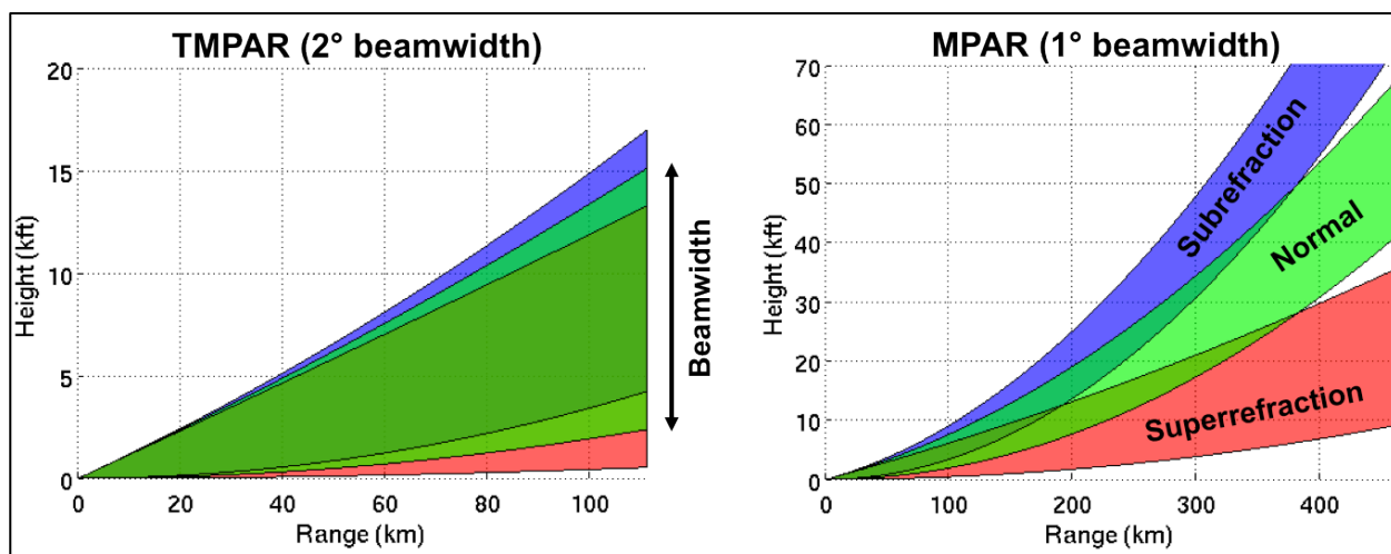
Figure 6-1. Terminal and Full-Scale MPAR beam height versus range for differing propagation conditions.
