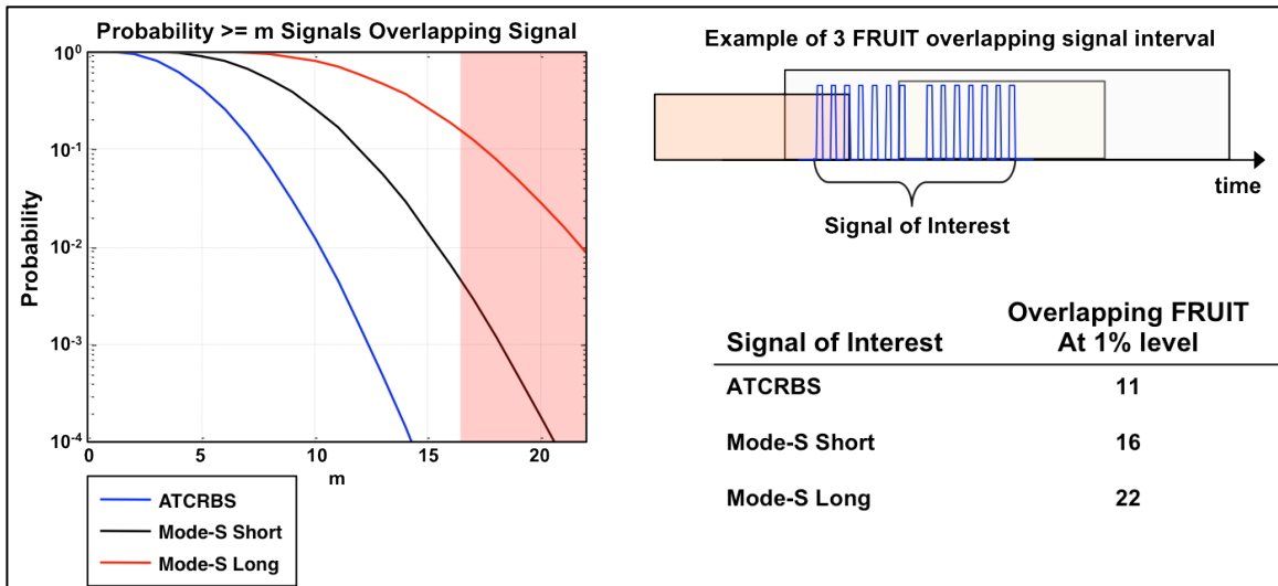
Figure 3-8. Signal overlap probability.
