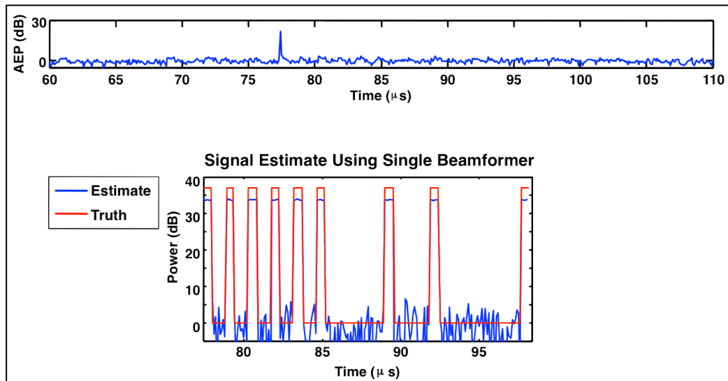
Figure 3-15. ATCRBS signal estimate.
