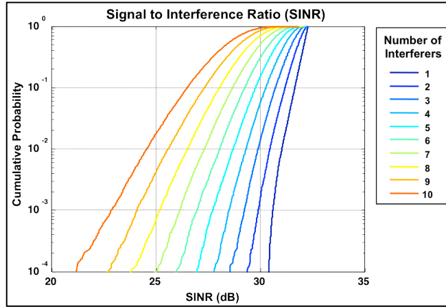
Figure 3-10. Cumulative probability for SSPAR array output signal to interference plus noise ratio.
