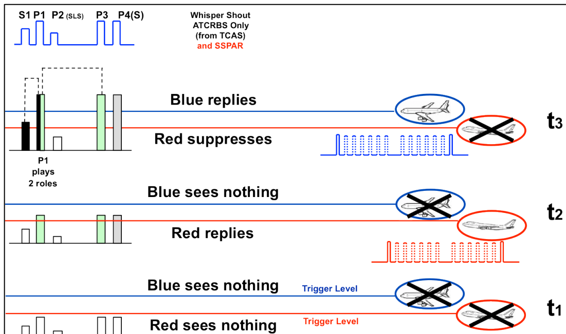
Figure 2-5. Whisper Shout interrogation for partitioning replies from closely spaced aircraft.
