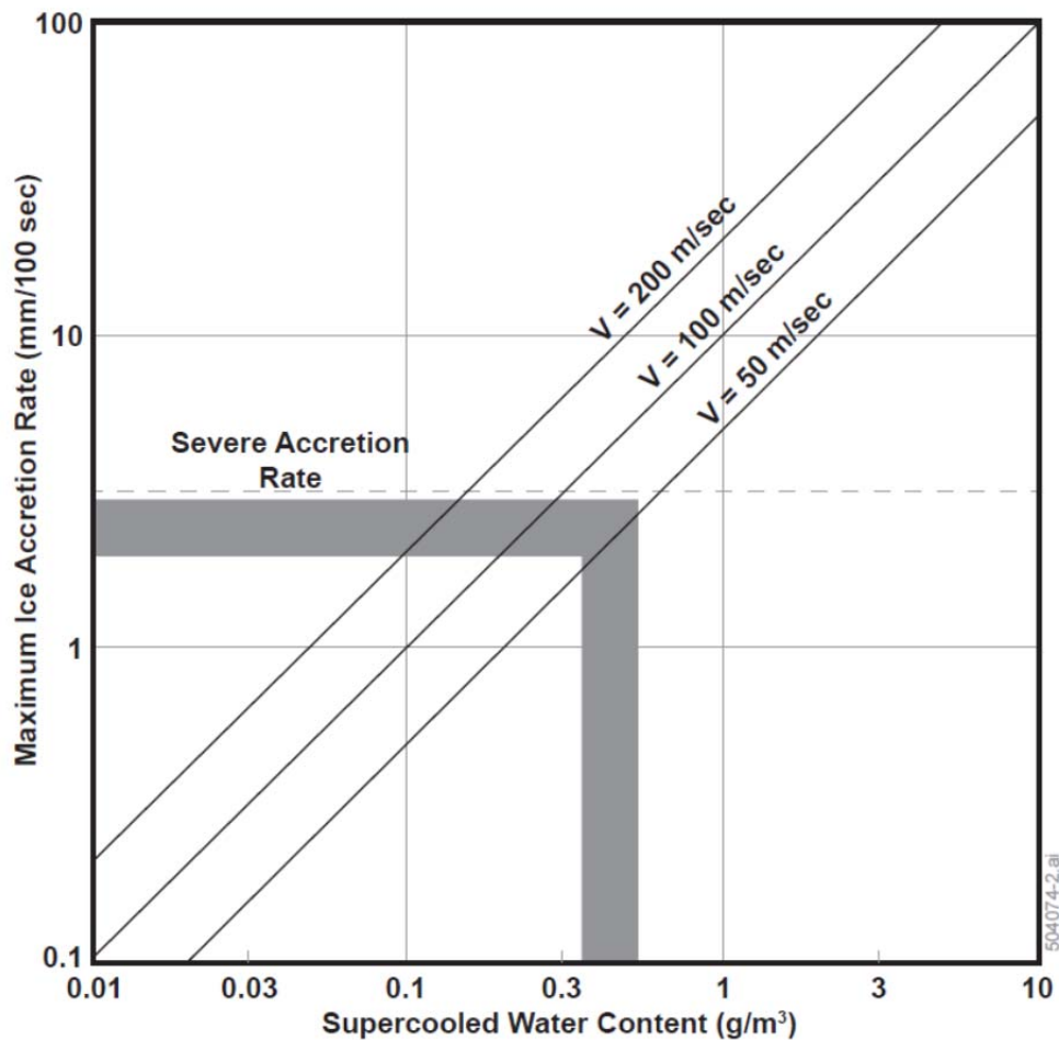
Figure 7-4. Comparison of estimated rime accretion rate with the theoretical predictions shown earlier in Figure 2-7 in Section 2 of this report. The gray region provides best estimates (and attendant uncertainty) for the icing situation with the Piper Archer aircraft on Feb. 21, 2013.
