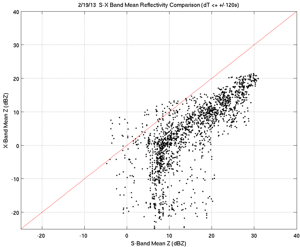
Figure D-3. Scatter plot of onboard X-band reflectivity and ground-based KBUF S-band reflectivity measured within \pm 120 seconds of the X-band measurement. These observations pertain to the flight on February 19, 2013. A +8 dB offset was used to correct the X-band data to force a match with the S-band observations, assumed to be well-calibrated (results shown in Figure 6-11).
