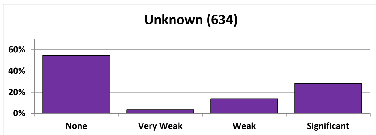
Figure 7-9. Distribution of SLW during aircraft encounters with HCA 'Unknown.'
