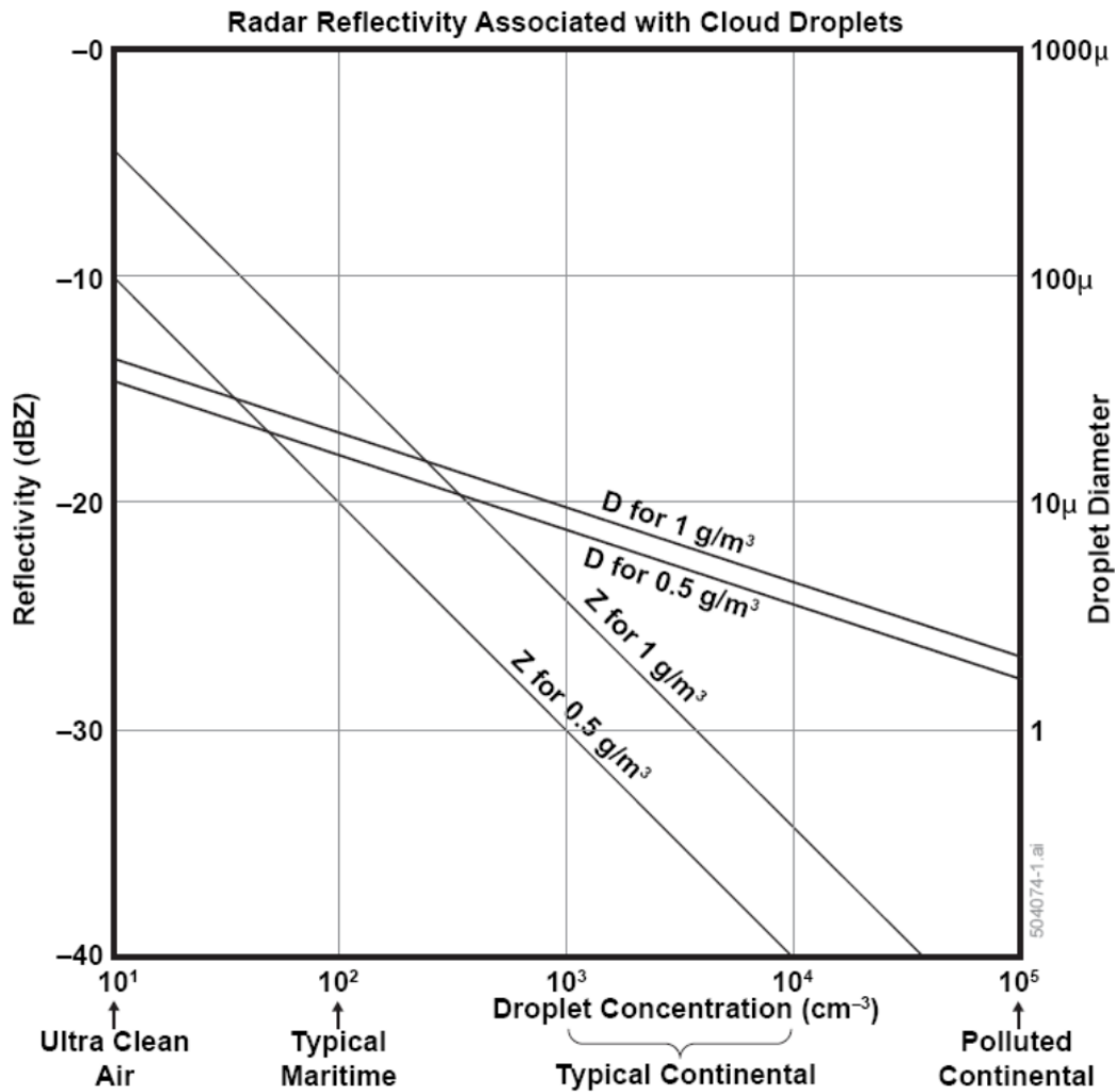
Figure C-1. Calculated radar reflectivity ( Z ) and cloud droplet diameter ( D ) based on the assumption that the available supercooled cloud water M (0.5 and 1.0 g/m 3 ) is shared amongst a concentration N of cloud droplets initiating on condensation nuclei.
