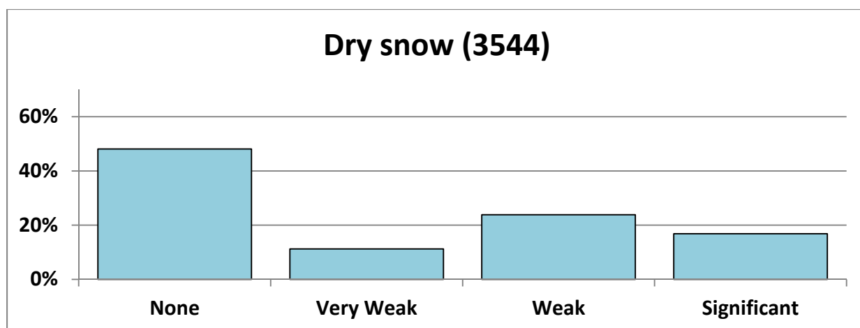
Figure 7-8. Distribution of SLW during aircraft encounters with HCA 'Dry Snow.'
