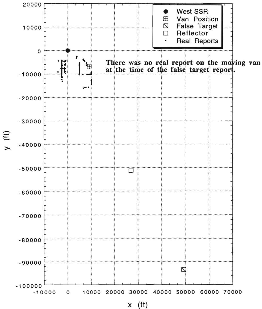
Figure 7c. ATCRBS false target report 49335, received by West SSR, operating in Mode S mode (Tue, 1/19/99).
