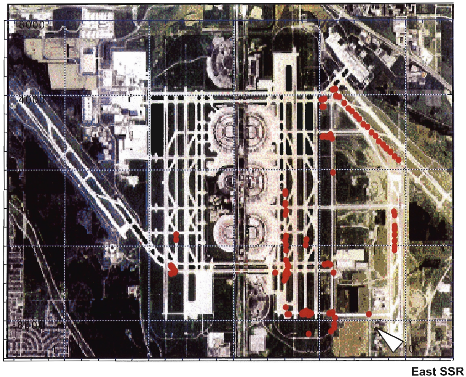
Figure 12. ATCRBS target reports, received by East SSR, operating in IBI mode, (Wed, 1/20/99).
