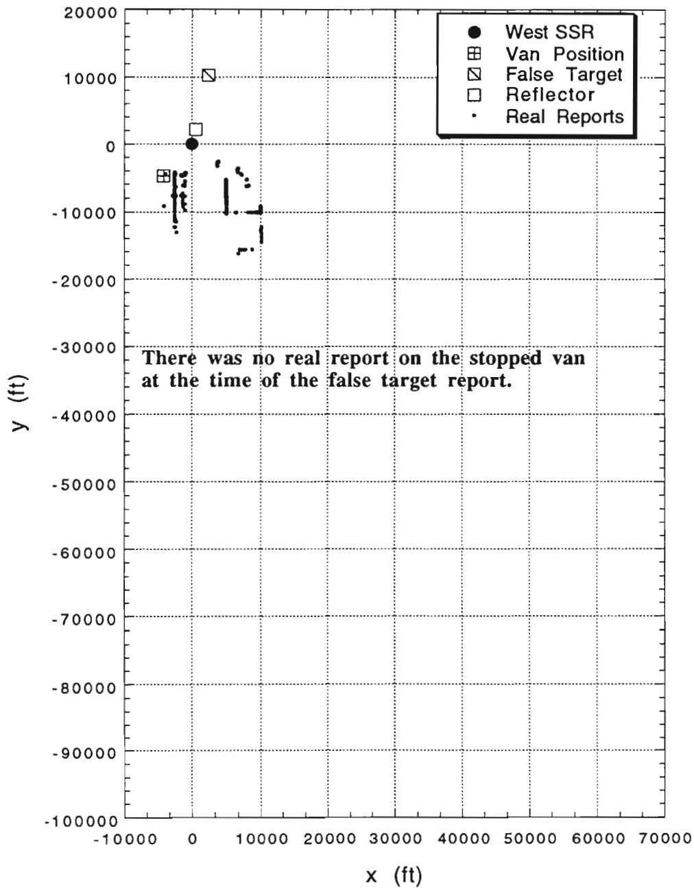
Figure 7e. ATCRBS false target report 2406, received by West SSR, operating in Mode S mode (Tue, 1/19/99).
