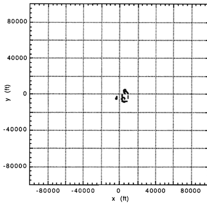
Figure 15. ATCRBS target reports to 100k ft, received by East SSR, operating in IBI mode (Wed, 1/20/99).
