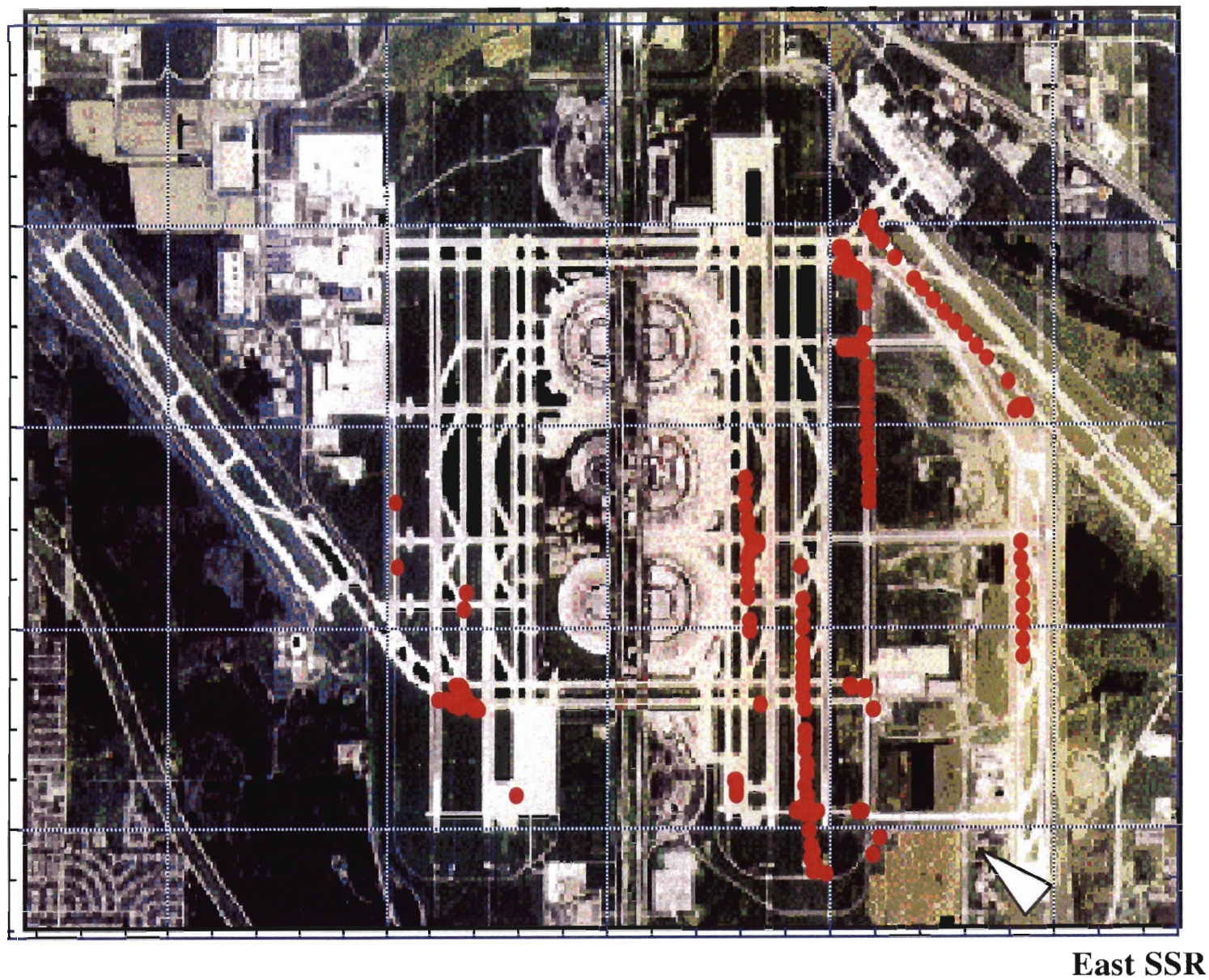
Figure 8. ATCRBS target reports, received by East SSR, operating in Mode S mode, (Wed, 1/20/99)
