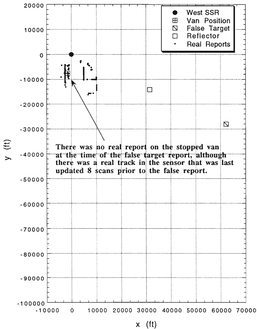
Figure 7d. ATCRBS false target report 62220, received by West SSR, operating in Mode S mode (Tue, 1/19/99).
