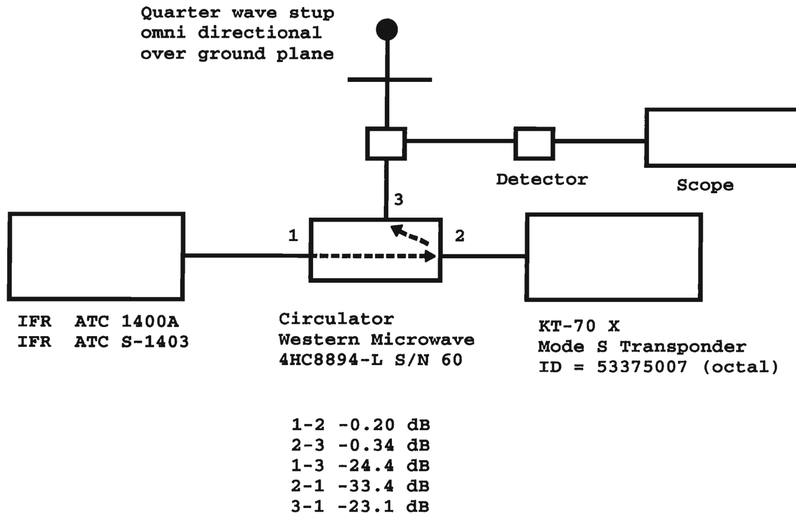
Figure 22. Re-interrogate Test Set Up.
