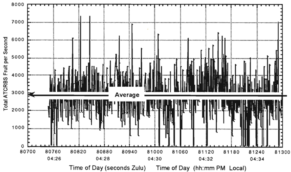
Figure 19. ATCRBS Fruit vs. Time.
