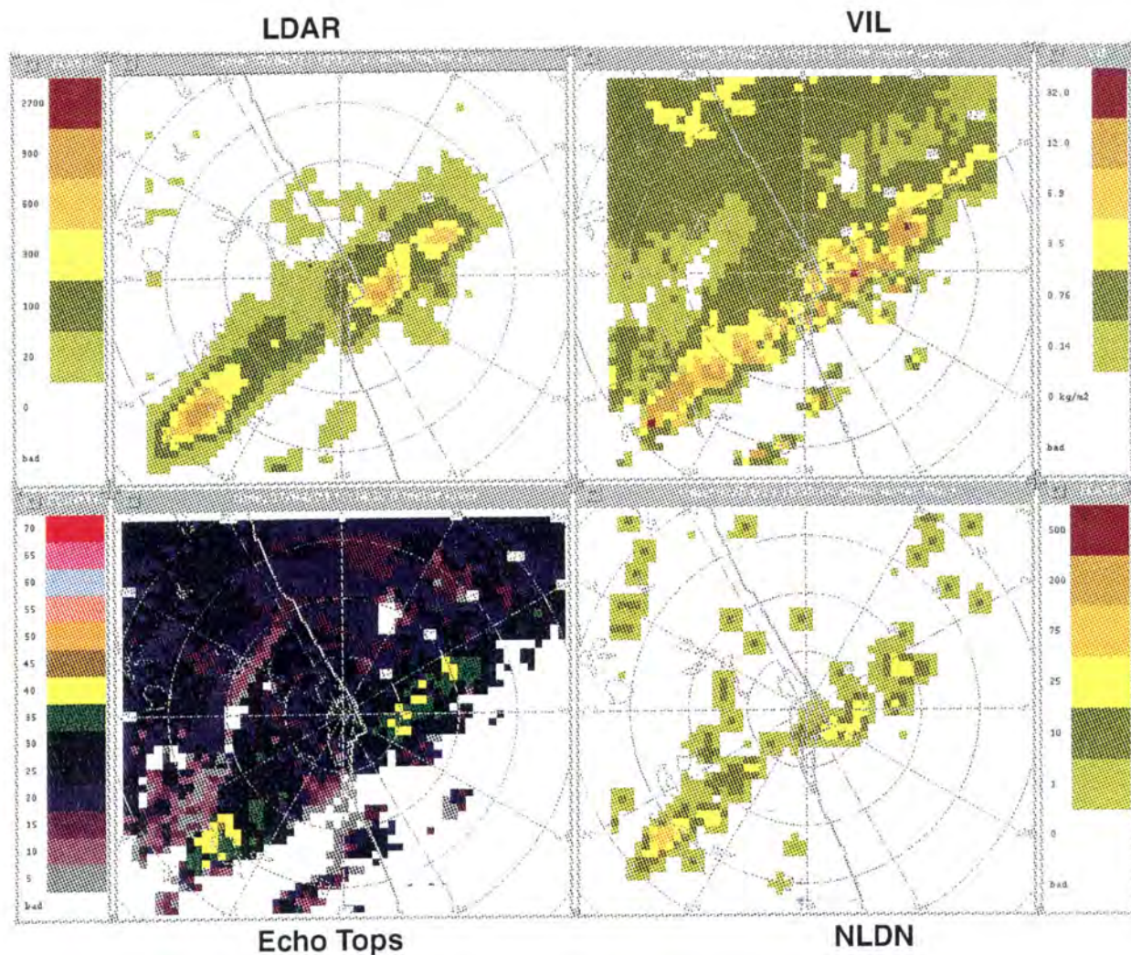
Figure 21. Four-panel plot showing LDAR, VIL and Echo Tops from NEXRAD, and NLDN data at 1638 UT on April 23, 1997. The lightning data has been mapped to two dimensions according to the procedure described in Appendix B. Lightning units are flashes per five-min. \times 48.8 (kernel weighting was not normalized). VIL units are \text{kg/m}^2 , and Echo Tops units are in kft.
