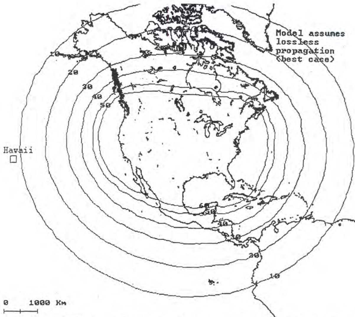
Figure 16. Map of NLDN detection efficiency in percent. Contours are in intervals of 10 percent (figure from Global Atmospherics, Inc.).
