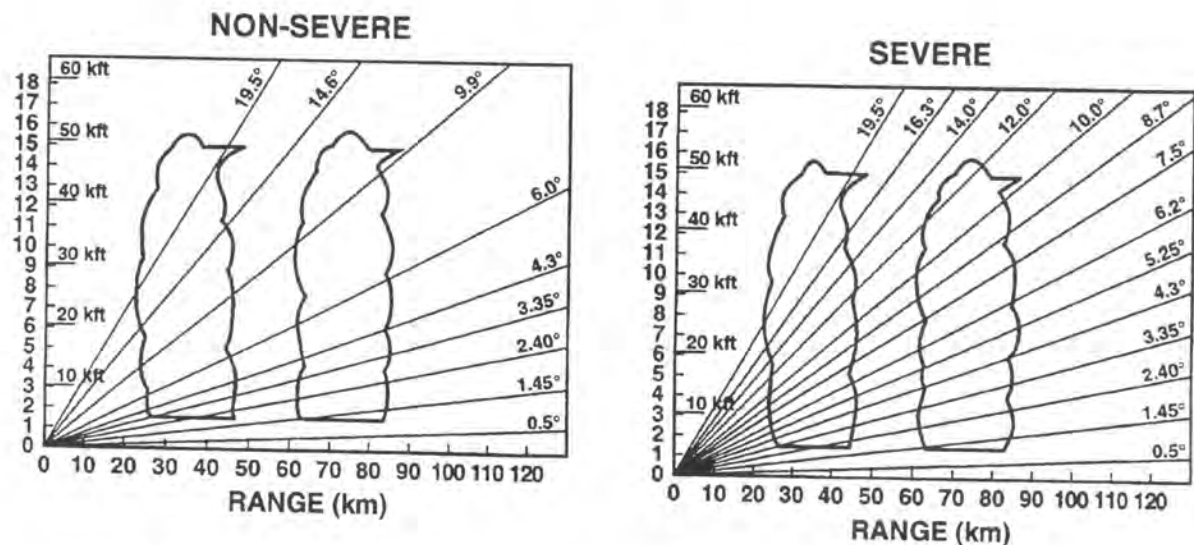
Figure 6. Comparison of NEXRAD scanning strategies in non-severe and severe weather conditions.
