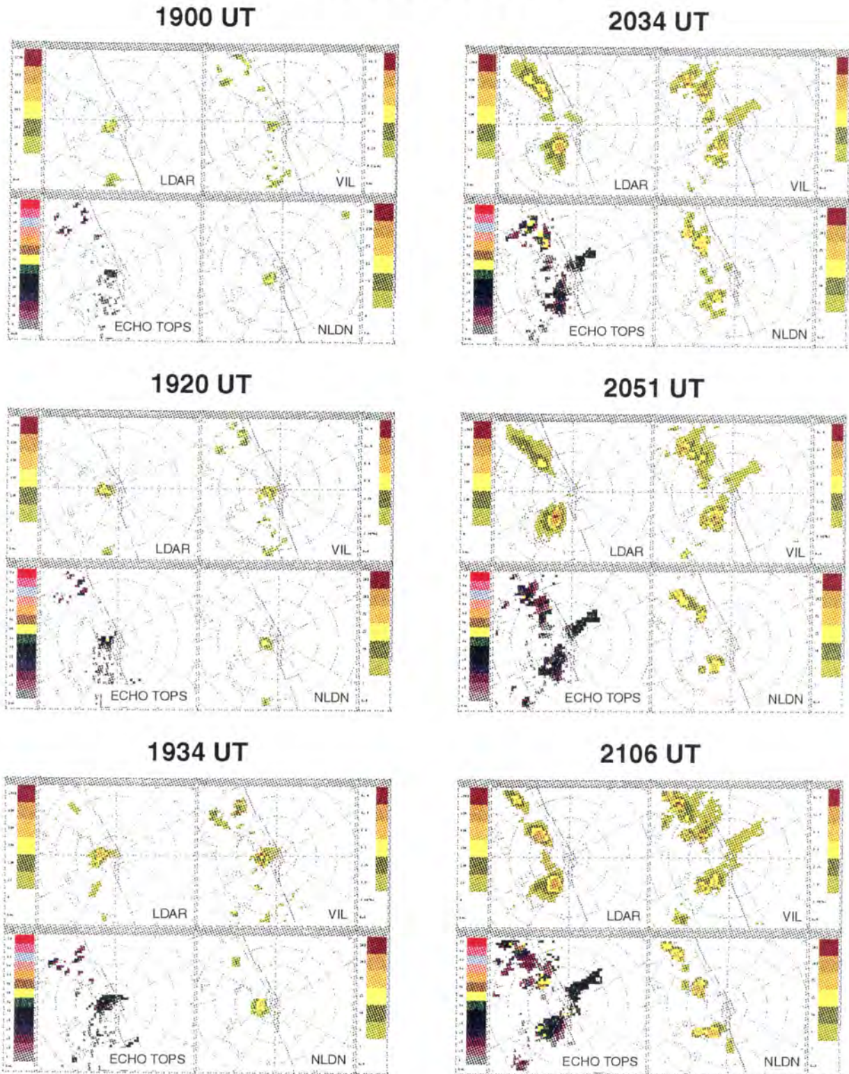
Figure 18. Six of the four-panel plots described in Figure 17 are shown for August 16, 1996. Images for every scan in the time interval shown in Table 17 are available from the authors at Lincoln Laboratory.
