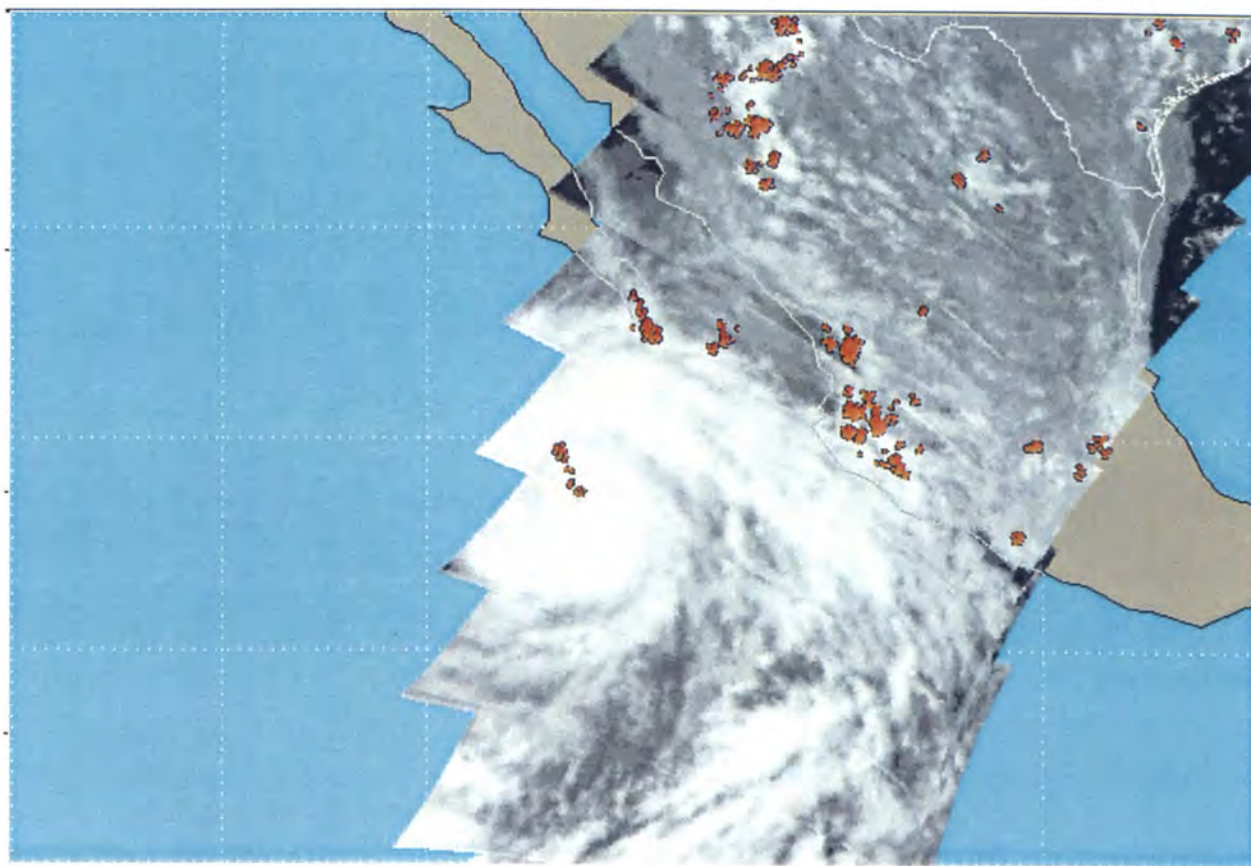
Figure C-1. Lightning flashes in the eyewall and rainbands of Hurricane Linda as observed by the NASA Optical Transient Detector on 12 September 1997. The flashes are superimposed on the OTD near-IR background images in the time interval 2115-2119 UTC. (Image courtesy of the NASA Global Hydrology and Climate Center, Huntsville, AL).
