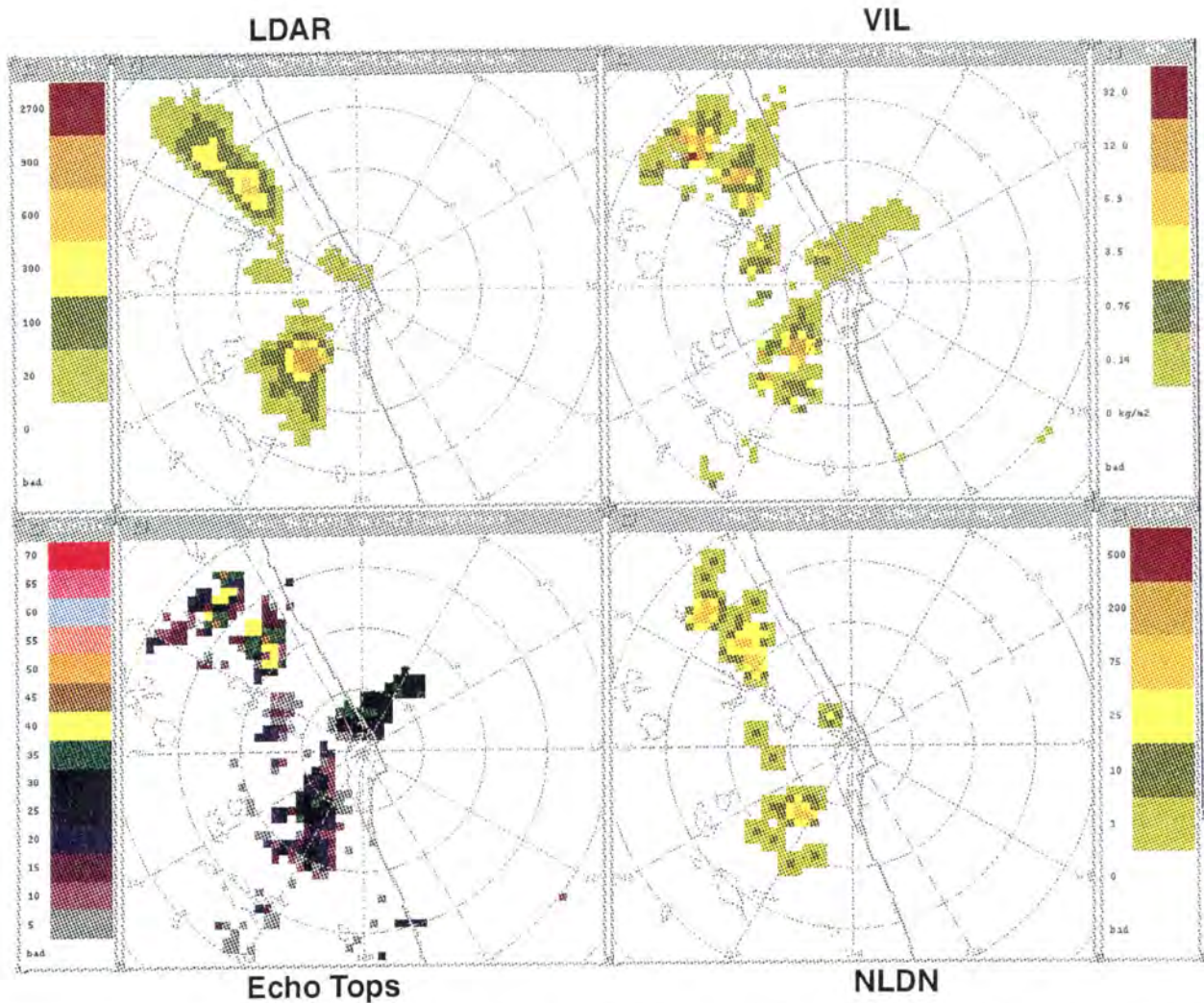
Figure 17. Four-panel plot showing LDAR, VIL and Echo Tops from NEXRAD, and NLDN data at 2034 UT on August 16, 1996. The lightning data has been mapped to two dimensions according to the procedure described in Appendix A. Lightning units are flashes per 5 min. \times 48.8 (kernel weighting was not normalized). VIL units are \text{kg/m}^2 , and Echo Tops are in kft.
