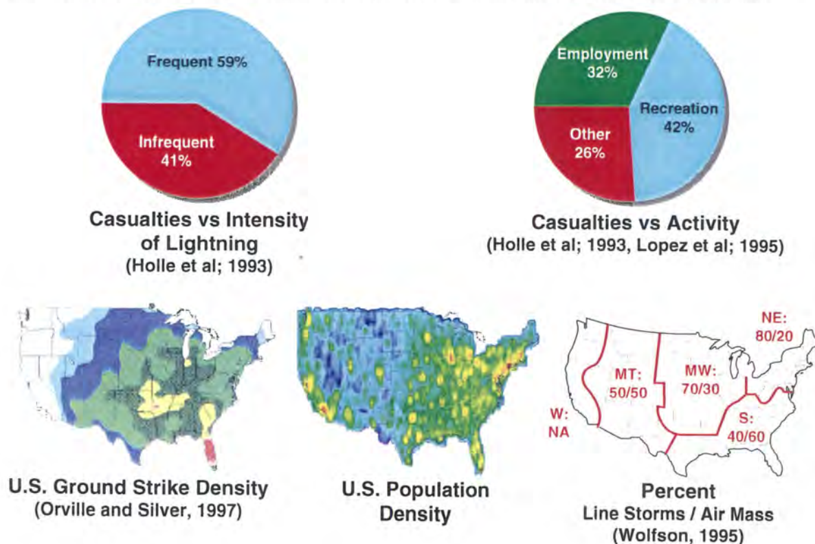
Figure 26. Data used in estimating LMS benefit for human warnings of lightning ground strike.
