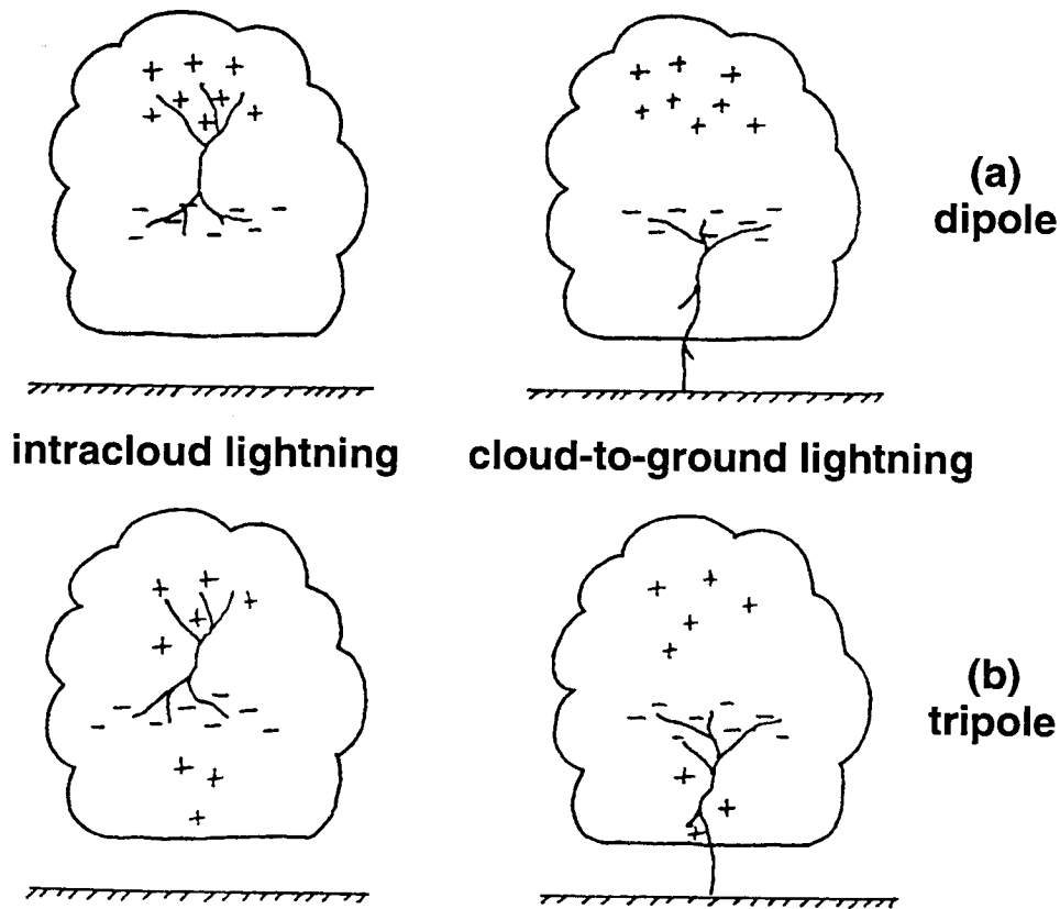
Figure 1. Depiction of intracloud and cloud-to-ground lightning in prototype electrostatic structures: (a) dipole and (b) tripole (from Williams, et al., 1989)
