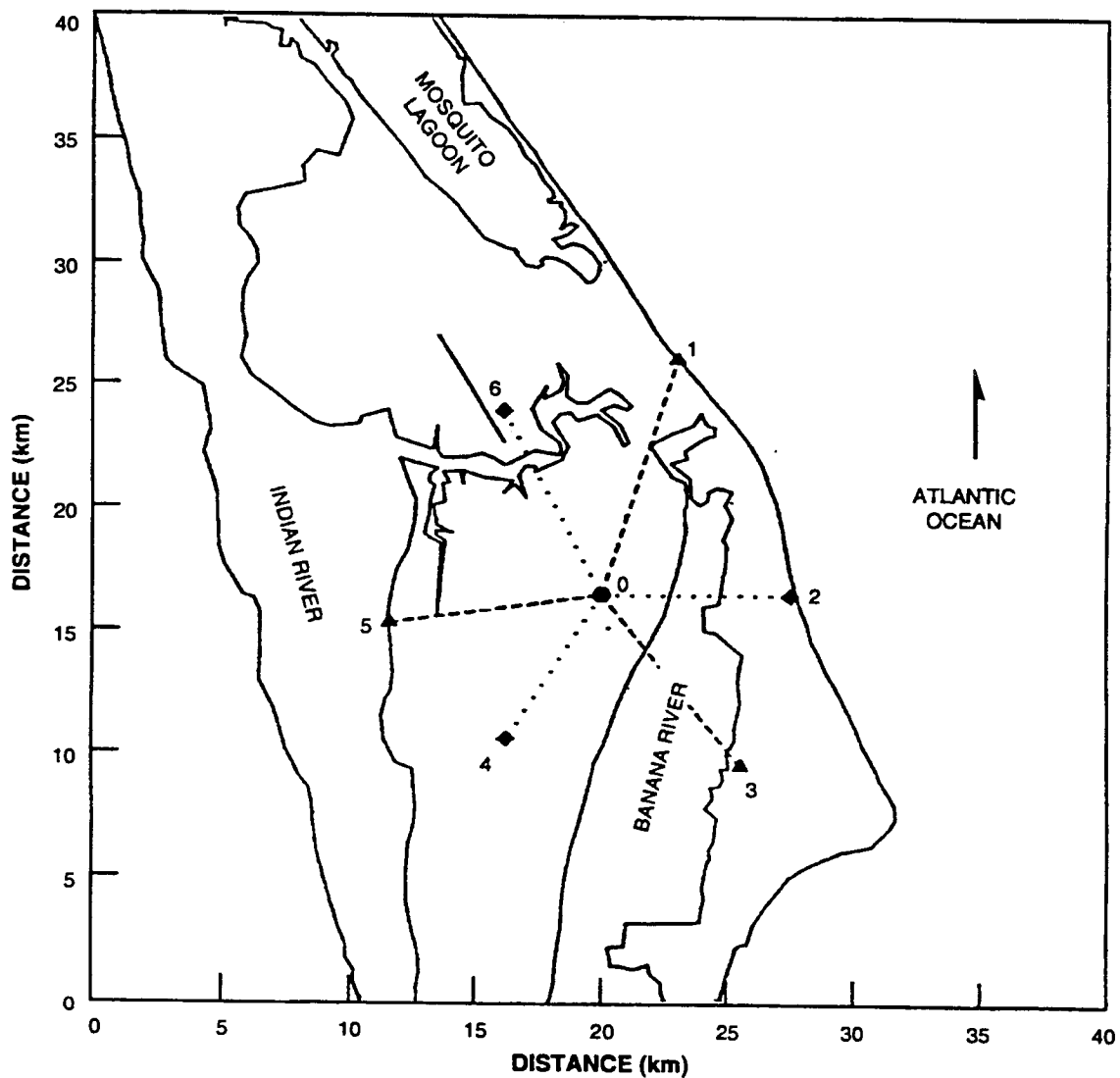
Figure 3. Antenna site locations for the Lightning Detection and Ranging (LDAR) system at Kennedy Space Center (adapted from Lennon and Maier, 1991).
