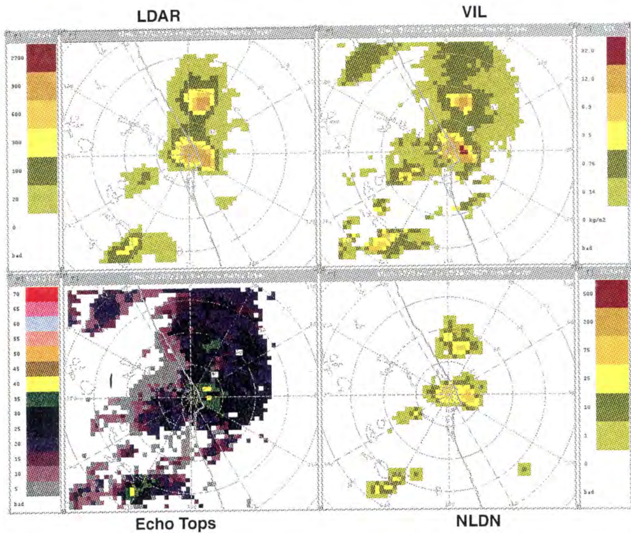
Figure 19. Four-panel plot showing LDAR, VIL and Echo Tops from NEXRAD, and NLDN data at 1941 UT on March 29, 1997. The lightning data has been mapped to two dimensions according to the procedure described in Appendix B. Lightning units are flashes per five-min. \times 48.8 (kernel weighting was not normalized). VIL units are \text{kg/m}^2 , and Echo Tops units are in kft.
