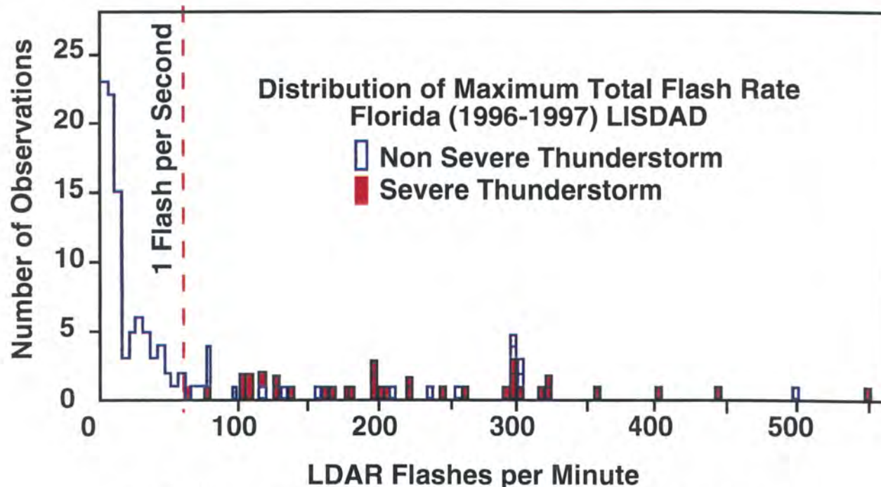
Figure 8. Histogram of maximum LDAR flash rate for nonsevere and for severe storms.
