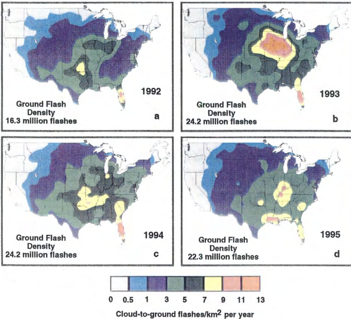
Figure 24. Lightning ground flash density for the years 1992-1995 are shown in panels (a) through (d), respectively. Measured values have been multiplied by 1.4 to correct for the assumed 70 percent detection efficiency in the NLDN (figure from Orville and Silver, 1997).
