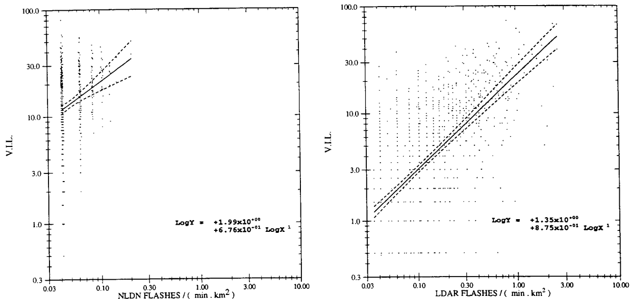
Figure 23. Linear regression between vertically integrated liquid water (VIL) pixel values and lightning flash rate densities.
