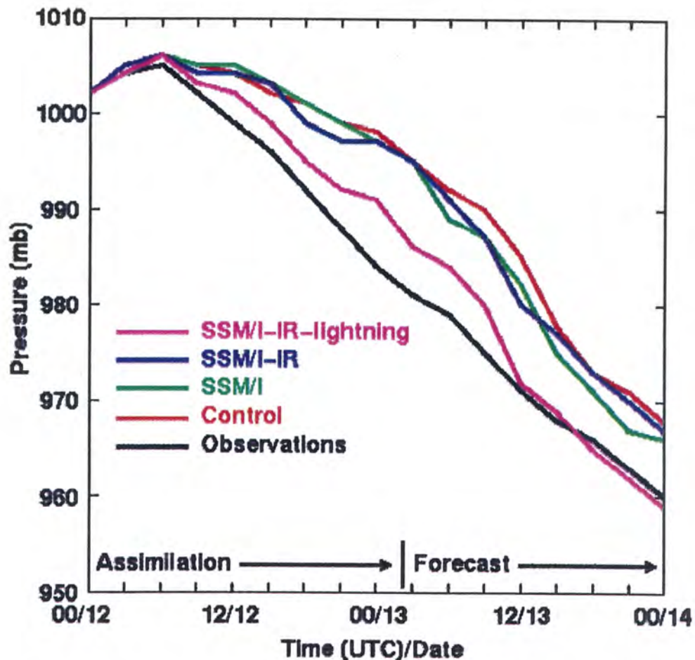
Figure C-2. Evolution of surface pressure of the 13 March 1993 Superstorm as a function of time, both during the assimilation period and the prediction period (Alexander, et al., 1997).
