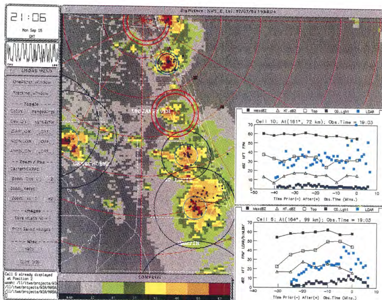
Figure 7. Operational LISDAD display at Melbourne, FL WFO.
