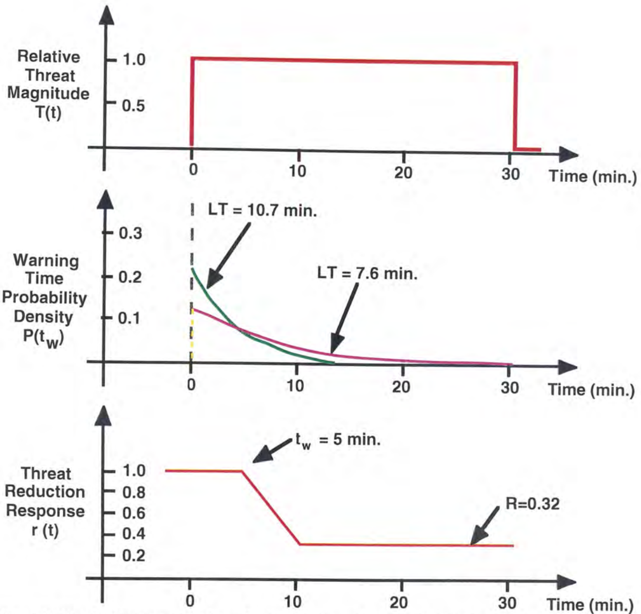
Figure 10. Warning/response model for evaluating LMS imposed warning benefits. Parameters are specific to the evaluation of tornado fatality reduction.
