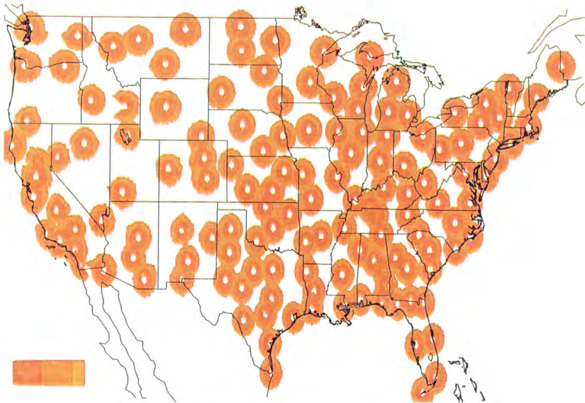
Figure 14 . NEXRAD three-dimensional coverage envelope as described in text.
