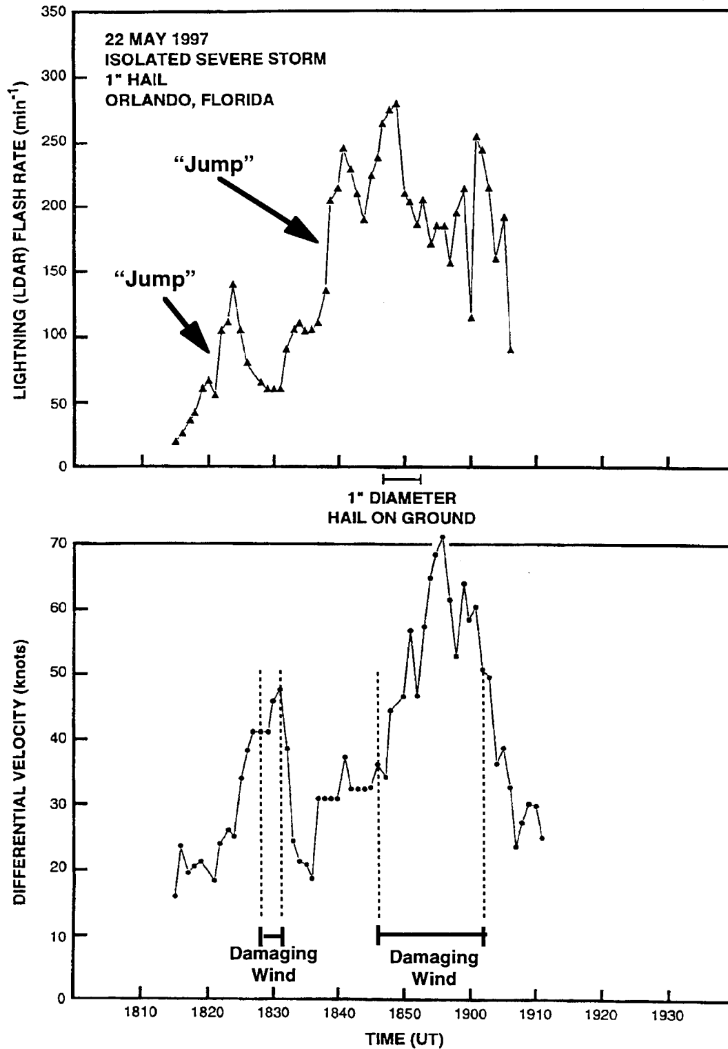
Figure 9. Evolution of LDAR flash rate (top) and differential radial velocity for a microburst-producing hailstorm on May 22, 1997.
