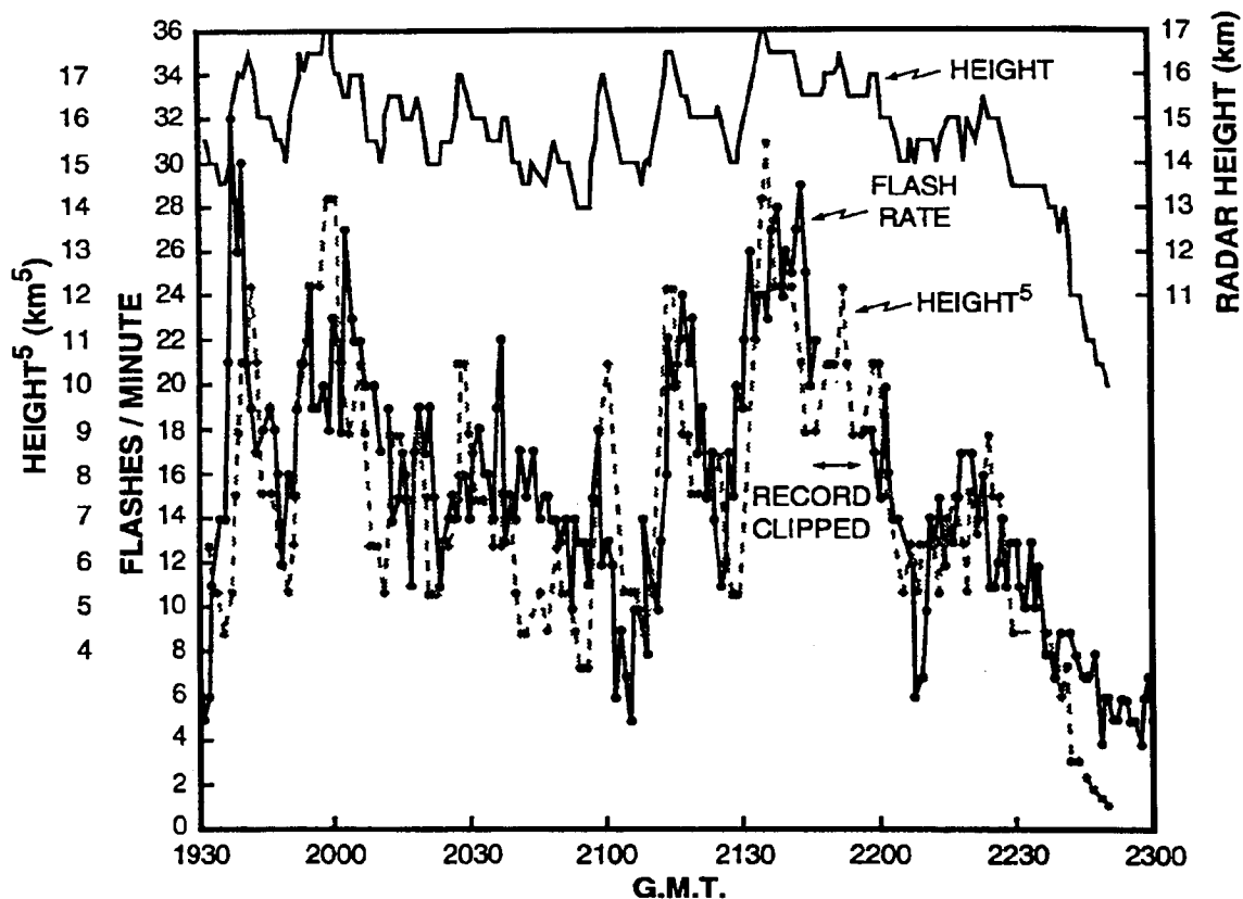
Figure 5. Comparison of total lightning flash rate and high-resolution radar measurements of cloud top height for a large Florida storm.
