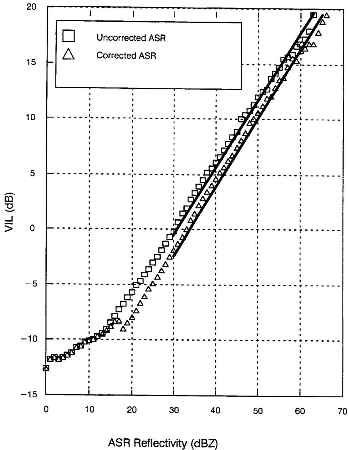
Figure B-1. Comparison of VIL and ASR reflectivity for uncorrected ASR reflectivity (boxes) and corrected ASR reflectivity (triangles), where the correction is applied only to reflectivities greater than 18 dBZ. (Troxel and Engholm, 1990.)
