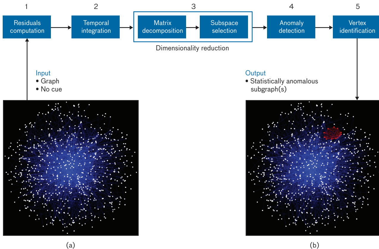
FIGURE 5. The Laboratory's Signal Processing for Graphs (SPG) framework is illustrated in the processing chain for uncued anomalous subgraph detection. A graph (a) in the form of an adjacency matrix is input into the chain. In steps 1 and 2, data are fit to the model, residuals are computed, and data are temporally integrated if necessary. In step 3, the dimensionality is reduced via a matrix decomposition. In steps 4 and 5, anomalous vertices are detected and identified. The final output is the subgraph (or subgraphs), as seen in (b).
