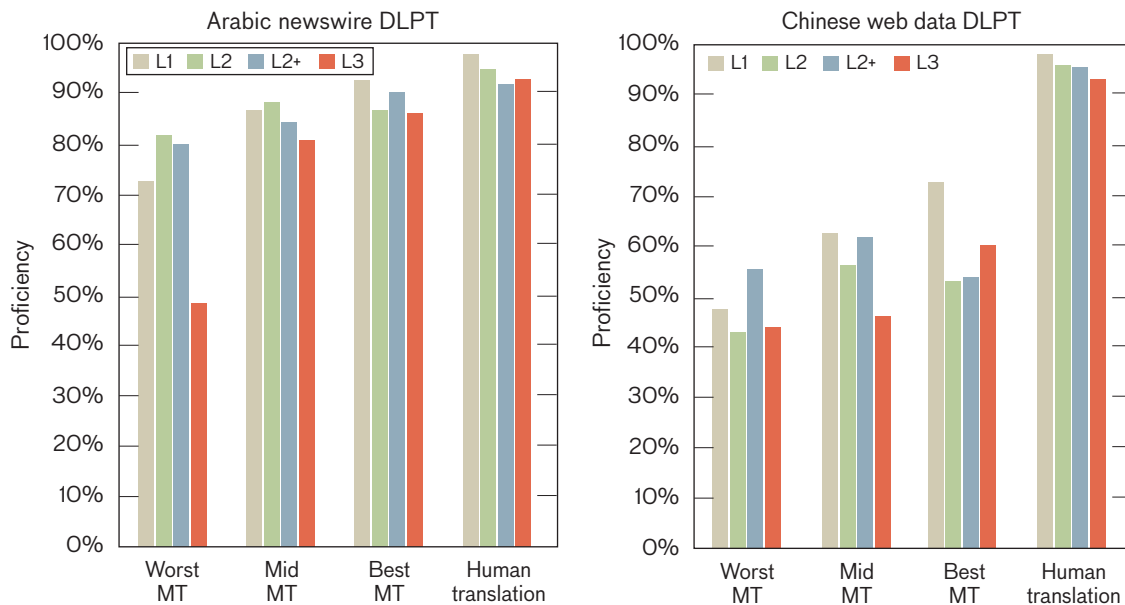
FIGURE 10. Two additional tests, developed in 2007, compared ten separate MT test conditions to reference translations. Performance for the best MT output of the ten systems, the worst of ten, and the system ranked fifth of ten are contrasted with the human translation. More difficult questions do follow the trend of achieving lower proficiencies for most of the tests, as expected, but there are some variations in the results. By comparing the results for the Arabic work on the left to the Chinese work on the right, it is clear that there is much more work to be done on the Chinese MT side.
