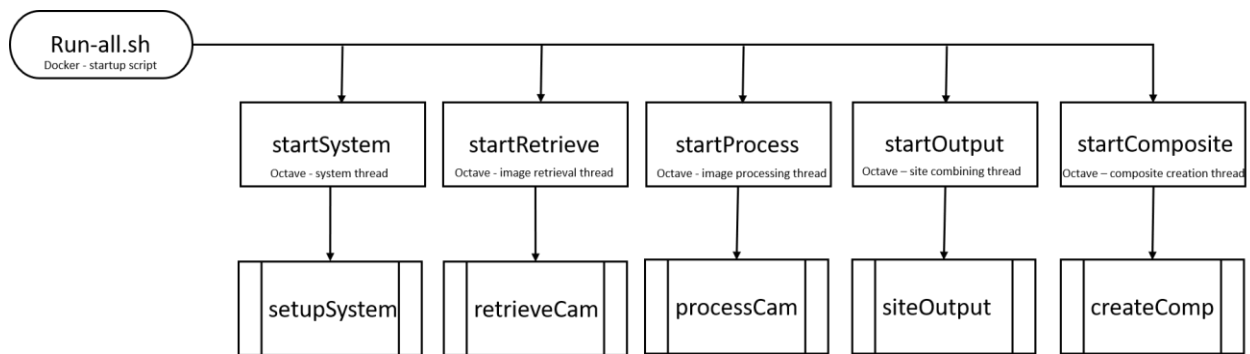
Figure 22. Top level flow chart of the VEIA processes. VEIA consists of five processes that execute simultaneously and are started from a shell script (Run-all.sh) within the docker file. All processes lead to an infinite loop that performs the desired actions on either a set strobe rate or at a specific time of day.
